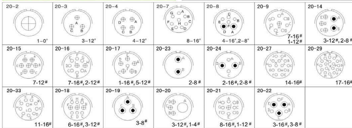
孔组排列 从插针方向看 Contacts Arrangement from Male Side
