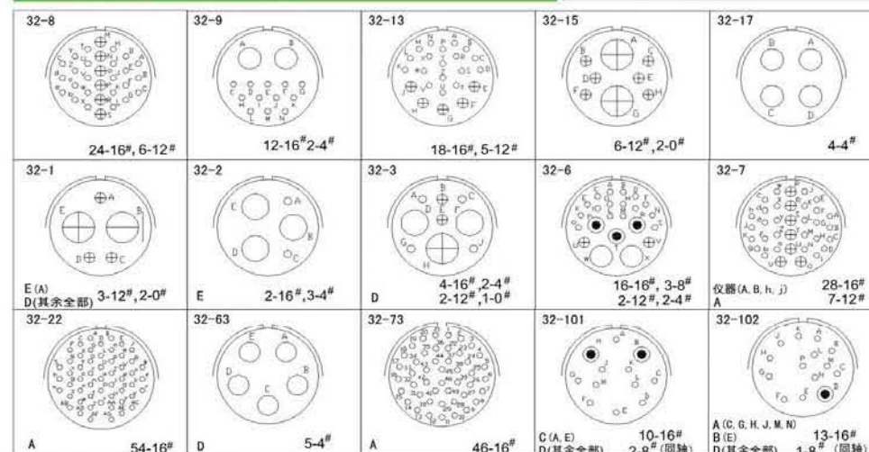
孔组排列 从插针方向看 Contacts Arrangement from Male Side
