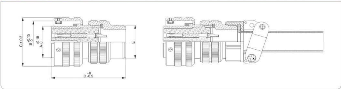
5015 3106 卡口直头图纸 5015 Bayonet Straight Plug Illustration
