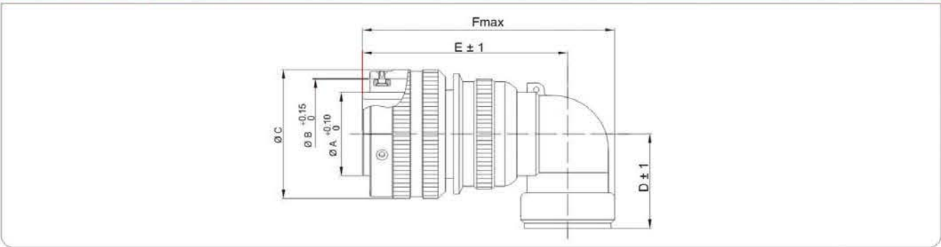
5015 3108卡口弯头图纸 5015 Bayonet 90°-Angle Plug Illustration
