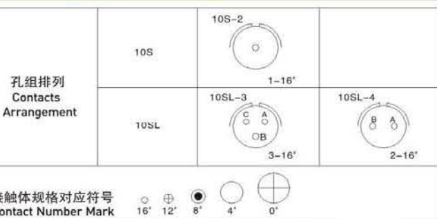
孔组排列 从插针方向看 Contacts Arrangement from Male Side
