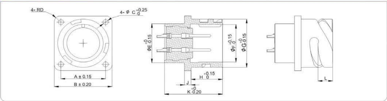
5015 3102卡口方座图纸 MS3102 Box Mounting Receptacle
