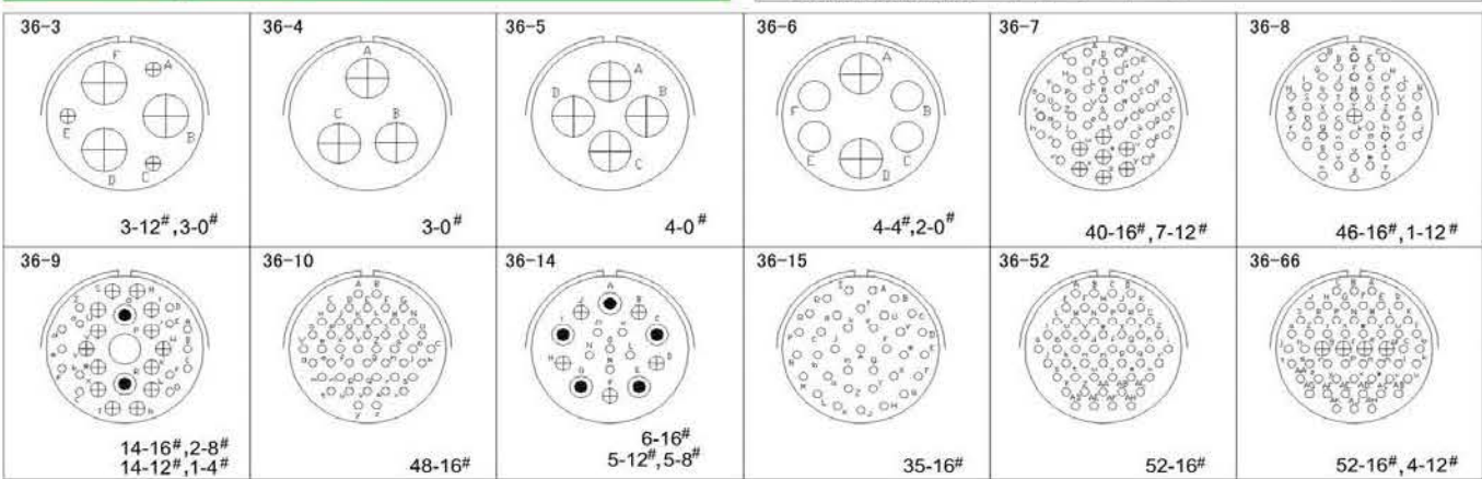
孔组排列 从插针方向看 Contacts Arrangement from Male Side
