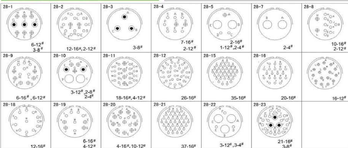
孔组排列 从插针方向看 Contacts Arrangement from Male Side
